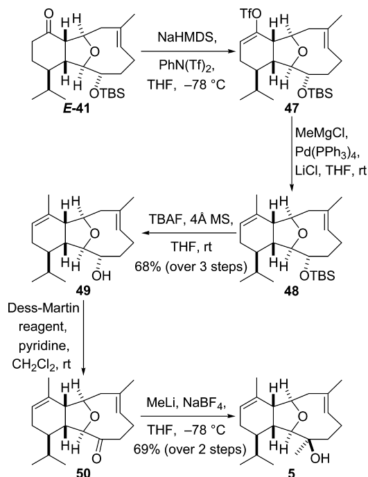
Scheme 14. Completion of Synthesis of the (-)-Cladiella-6,11-dien-3-ol ( 5 )
