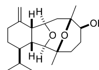
Figure 4. Structure originally proposed for sclerophytin A.
